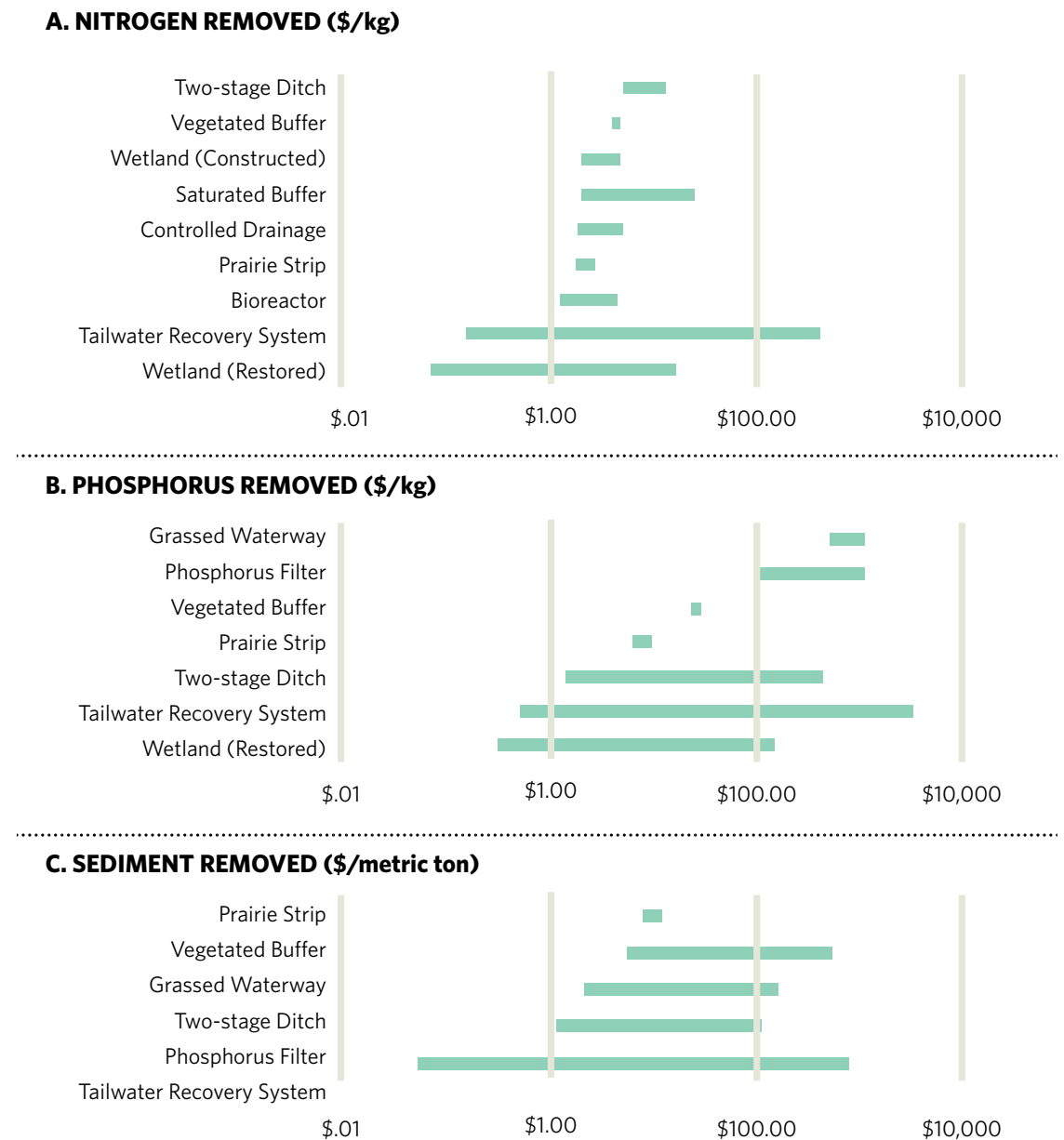
Figure 4A-C. Cost-effectiveness of EoF practices for nitrogen, phosphorus, and sediment removal
